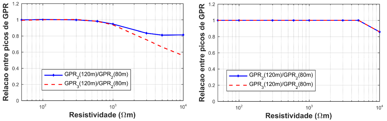
(a) GPR_{2(120m)}/GPR_{2(80m)} e GPR_{3(120m)}/GPR_{2(80m)}
