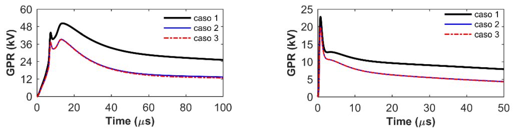
(a) 50 \Omega\text{m}
