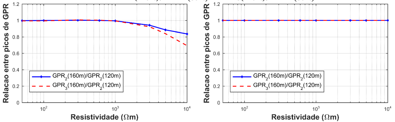
(b) GPR_{2(160m)}/GPR_{2(120m)} e GPR_{3(160m)}/GPR_{2(120m)}
